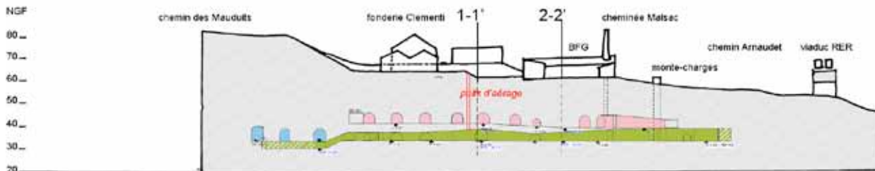
SECTION B-B'
